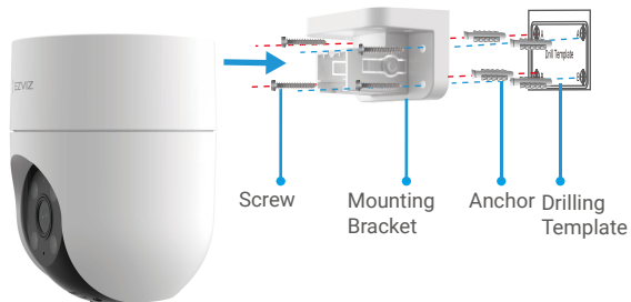
Fig. 2 Wall Mount
